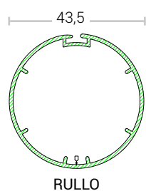
RULLO
